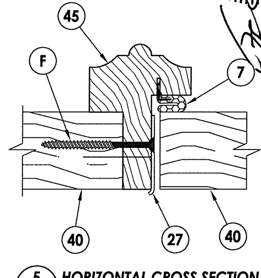
5 HORIZONTAL CROSS SECTION 3 Outswing shown (Inswing similar)
