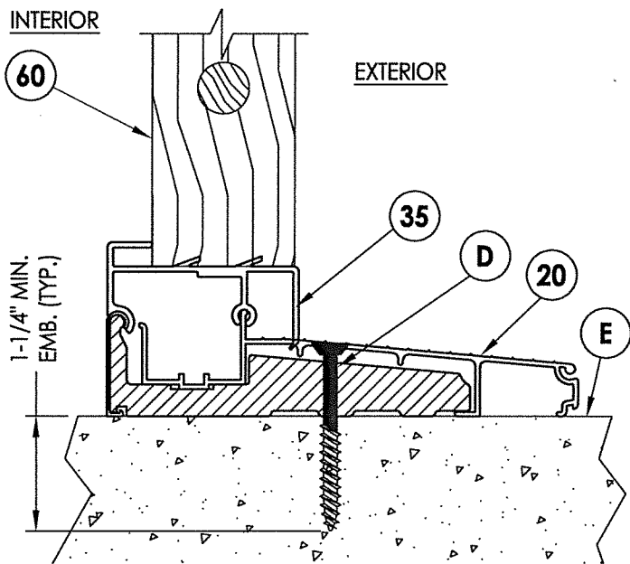
5 4 VERTICAL CROSS SECTION Inswing sill
