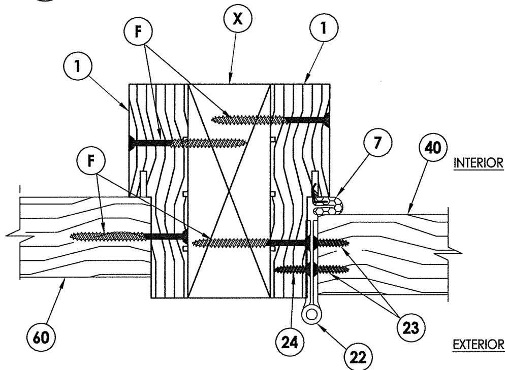
3 HORIZONTAL CROSS SECTION 3 Outswing shown (Inswing similar)
