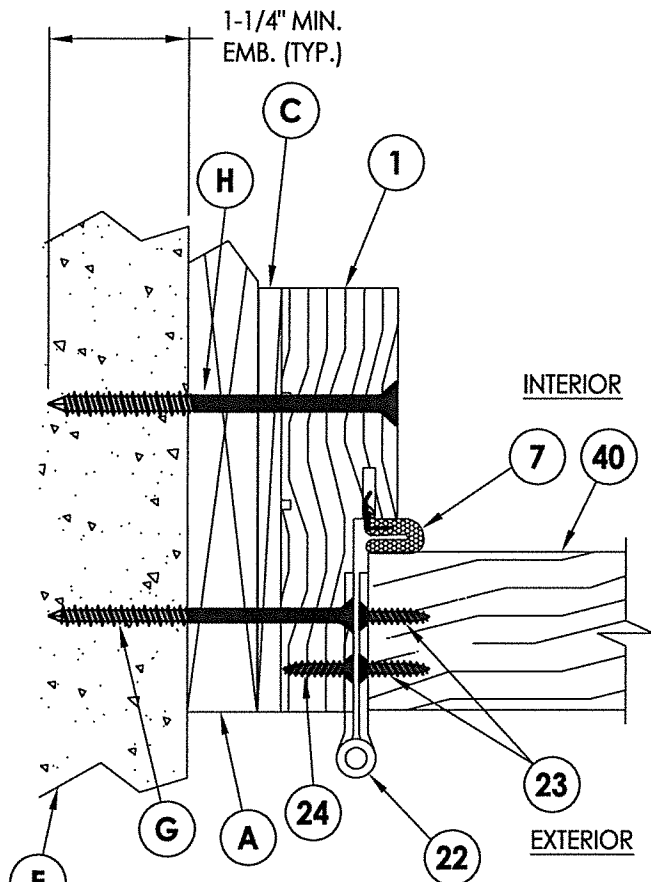
1 HORIZONTAL CROSS SECTION 3 Shown w/1X sub-buck
