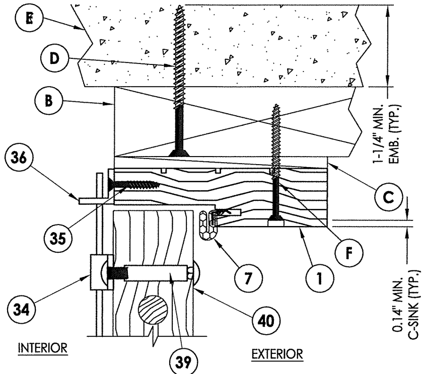
1 4 VERTICAL CROSS SECTION Inswing shown
