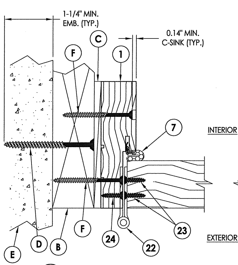
2 HORIZONTAL CROSS SECTION 3 Outswing shown (Inswing similar)
