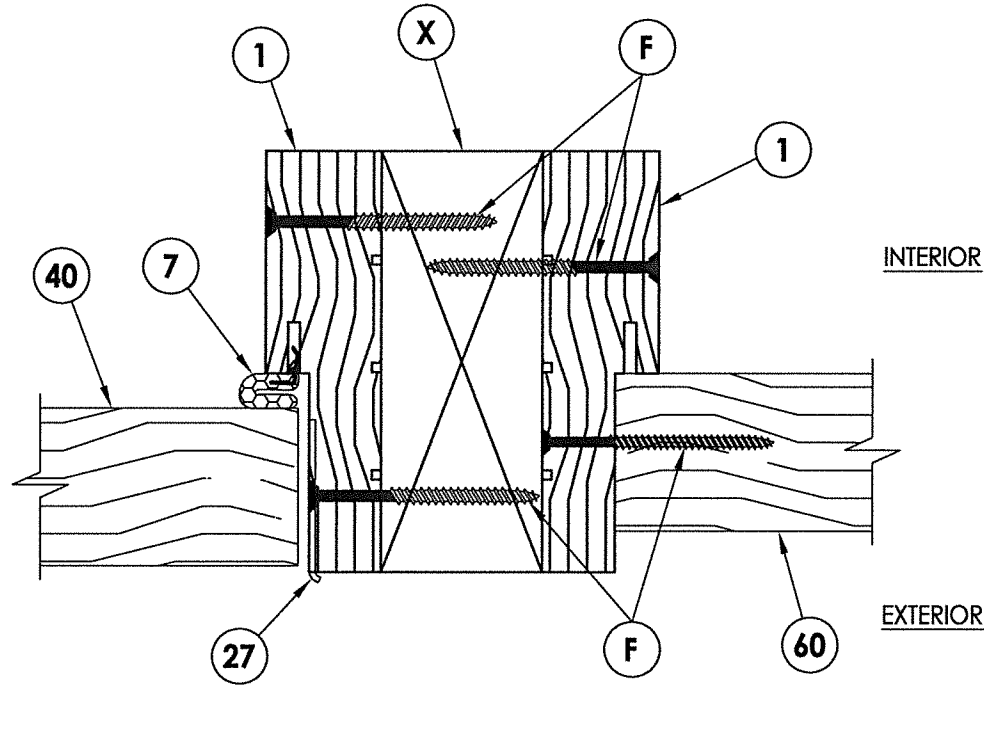
4 HORIZONTAL CROSS SECTION 3 Outswing shown (Inswing similar)
