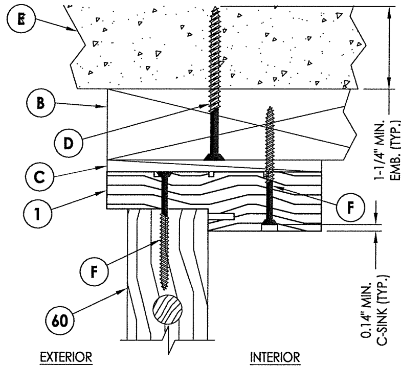
3 4 VERTICAL CROSS SECTION Outswing shown
