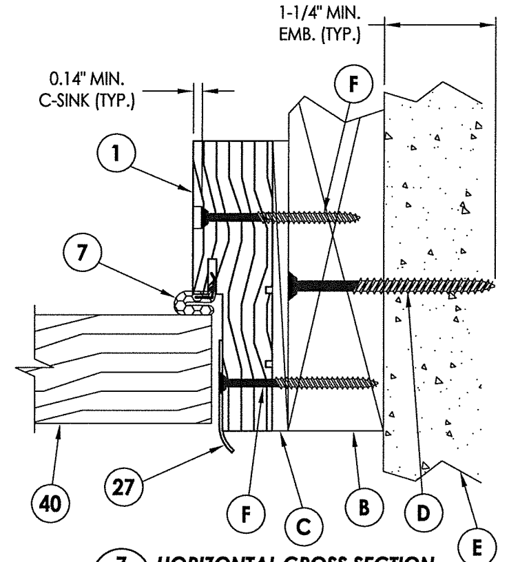
7 HORIZONTAL CROSS SECTION 3 Outswing shown (Inswing similar)
