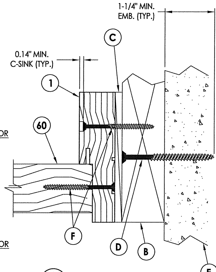
6 HORIZONTAL CROSS SECTION 3 Outswing shown (Inswing similar)
